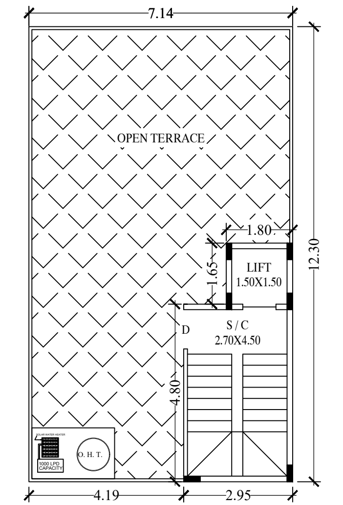
PROPOSED TERRACE FLOOR PLAN
